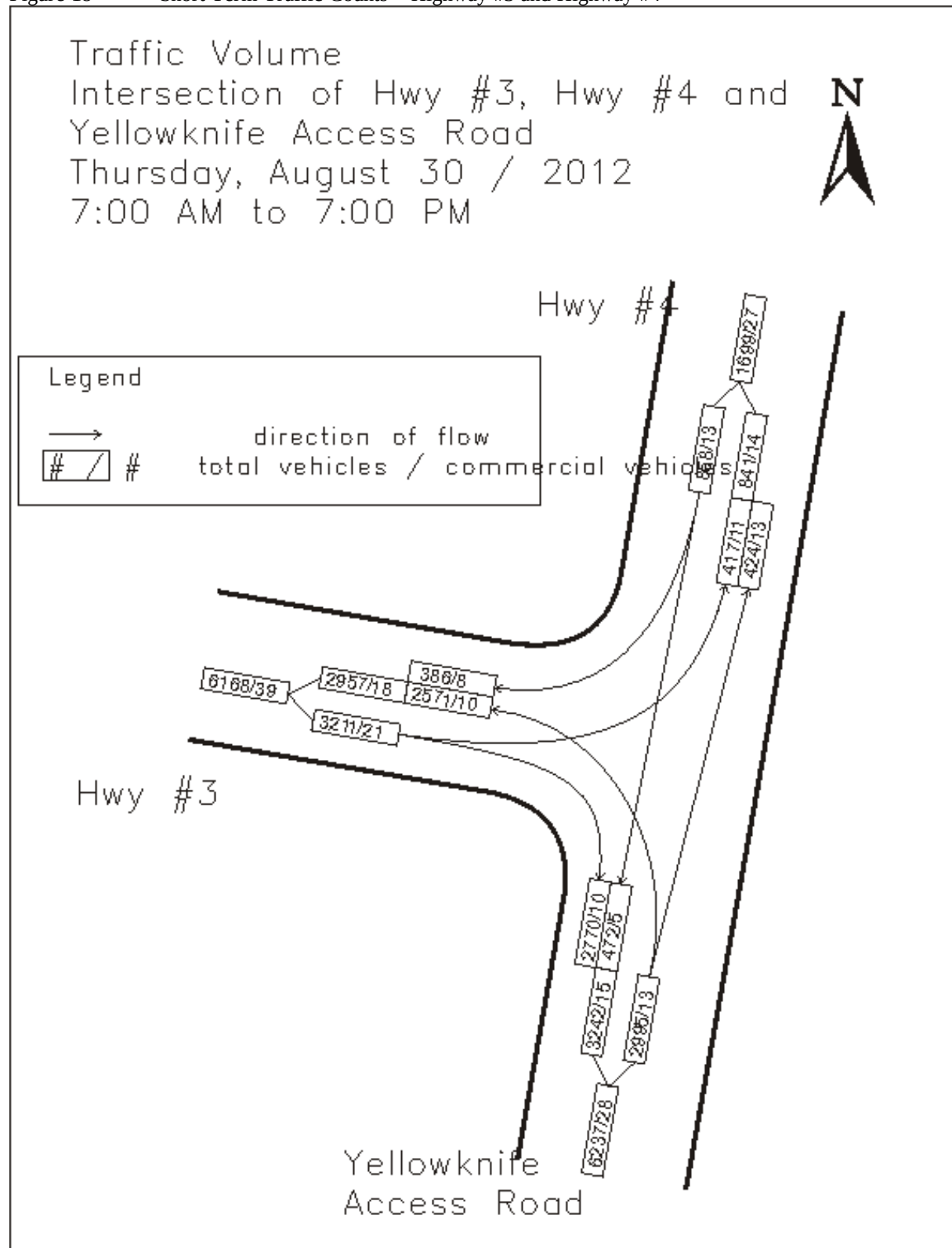
Figure 18 Short Term Traffic Counts – Highway #3 and Highway #4
