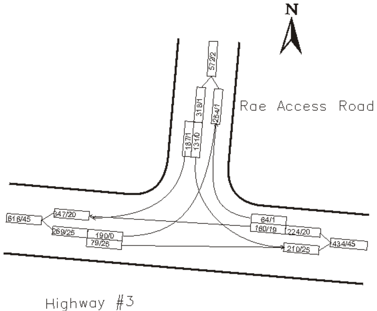
Figure 16 Short Term Traffic Counts – Highway #4 and Rae Access Road
